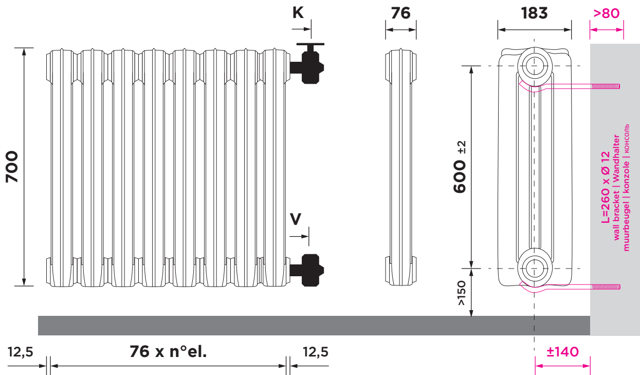
on the wall | wandhängend | muurhangend | на зди | на стене AD760-W, all dimensions in mm ±2
