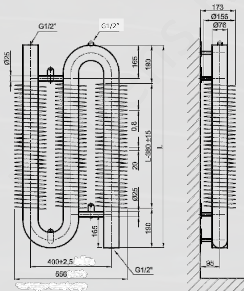
RA03 76×2,5×156 VERTICAL RIGHT
